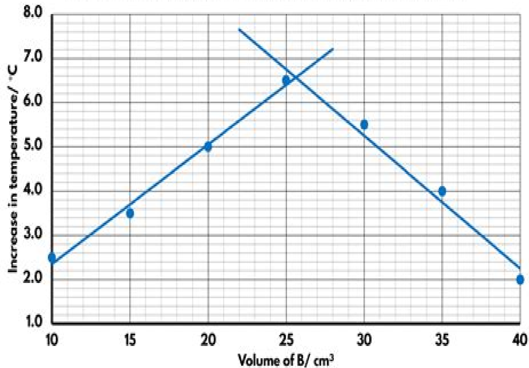
Graph of temperature increase/ ^{\circ}\text{C} against volume of B/ \text{cm}^3
