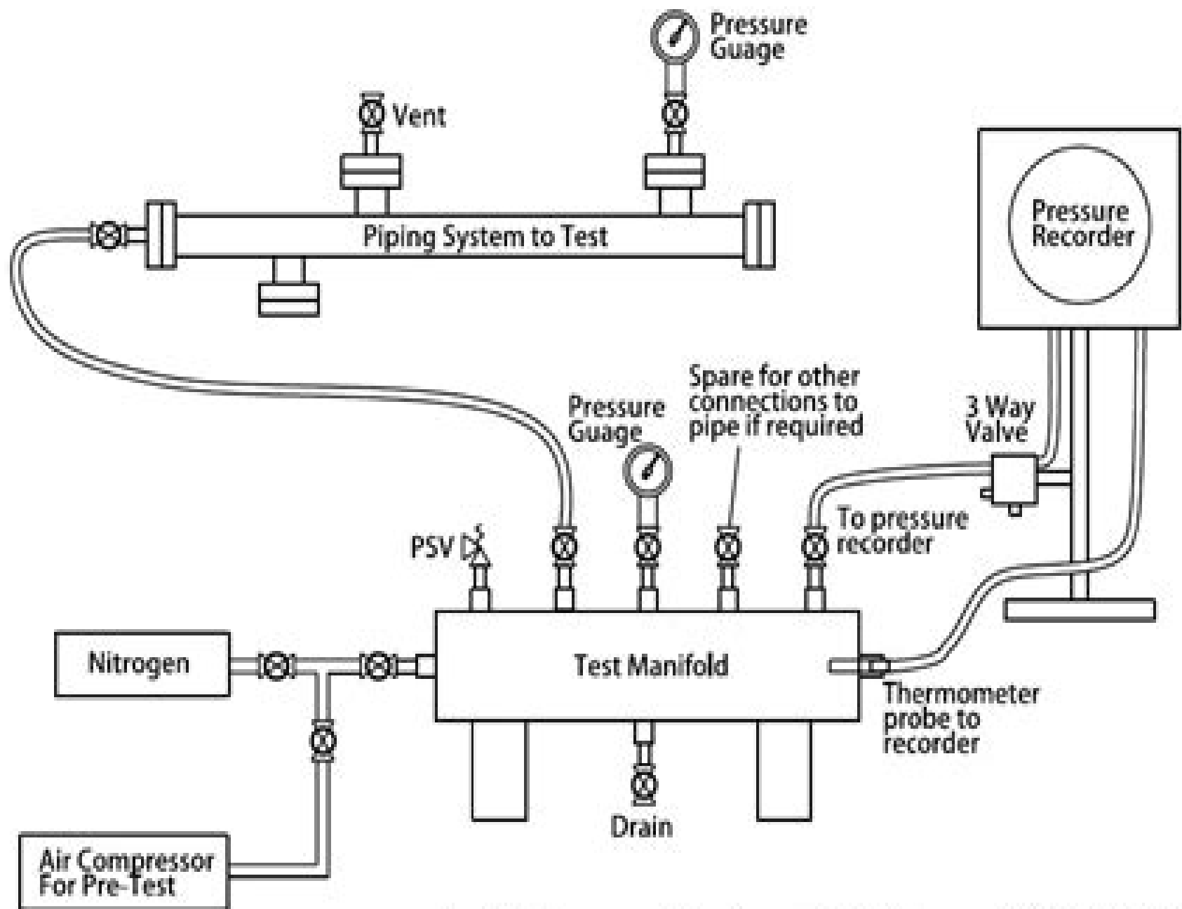
Manifold Arrangement for Pneumatic Testing
