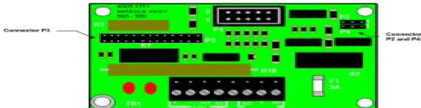
Figure 1. 4005 City Circuit Card
