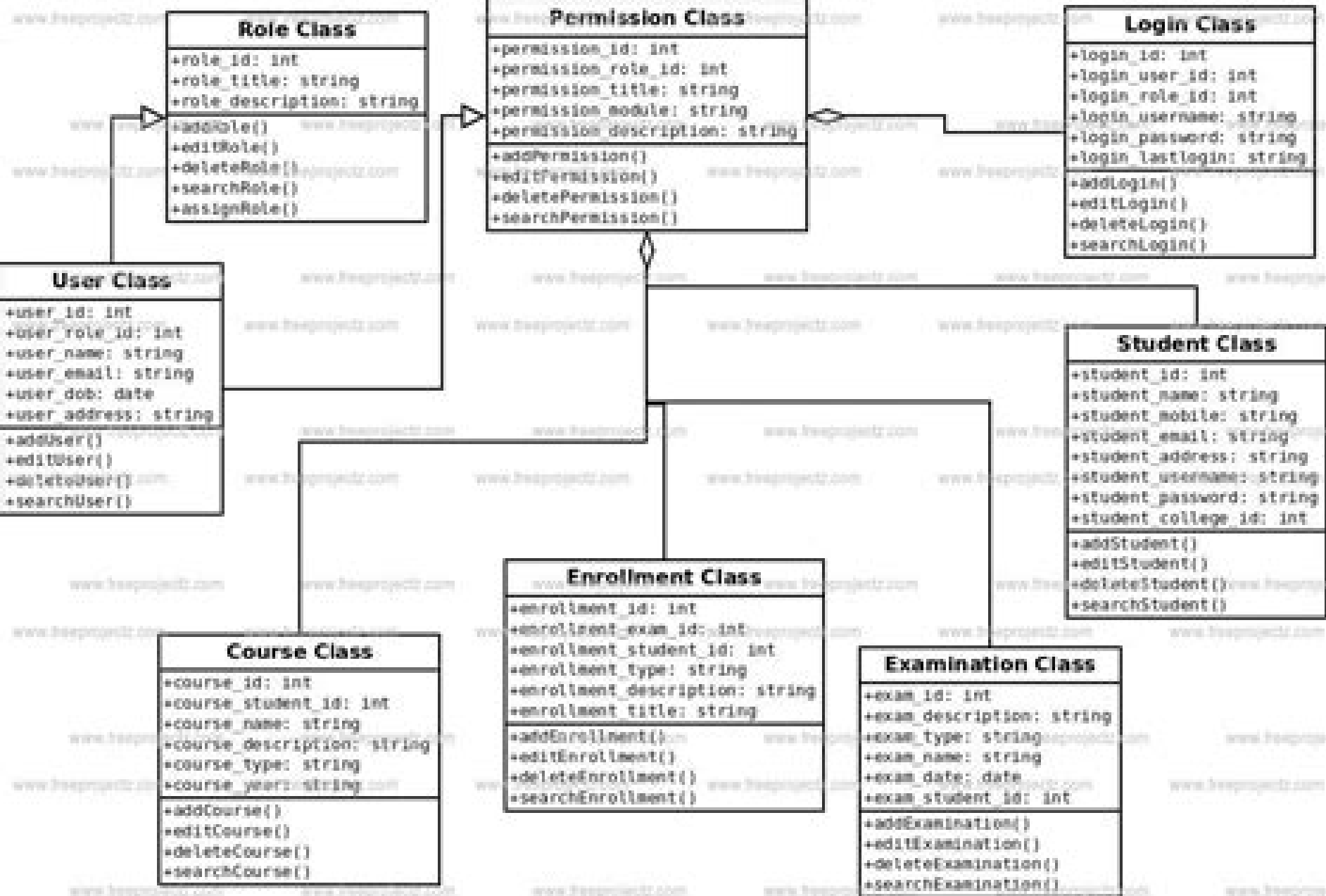
Class Diagram of Enrollment System
