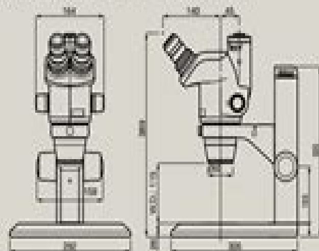
SMZ745T set SMZ745T + C-PSN Plain Stand (CN)
