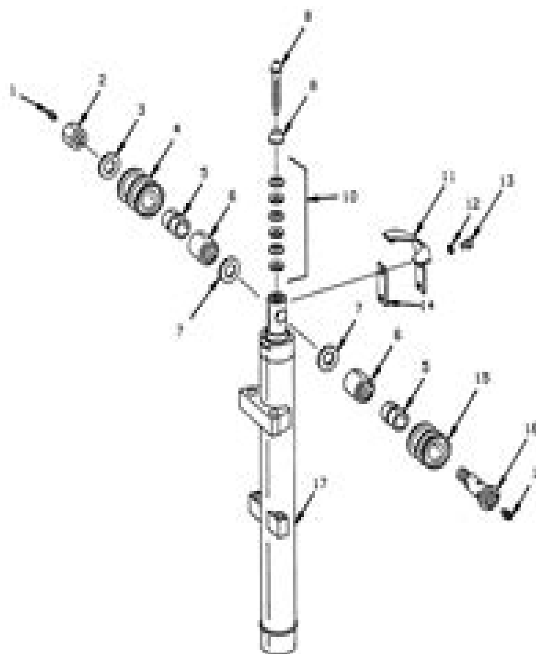
FIGURE 4 TO THREE STAGE FREELIFT CYLINDER INSTALLATION
