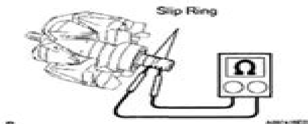
Fig. 32: Measuring Resistance Between Slip Rings
