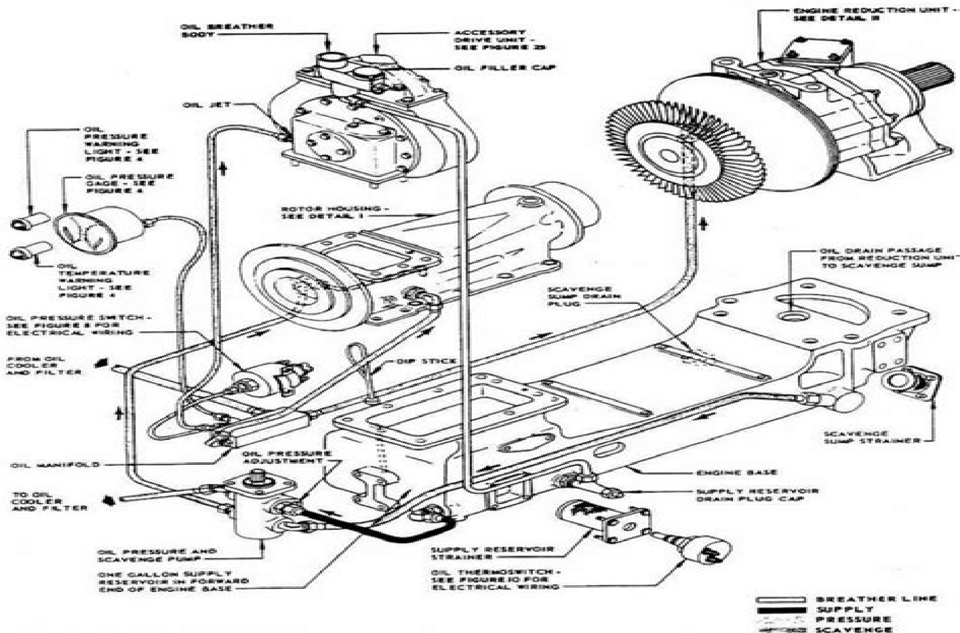
Engine Oil System
