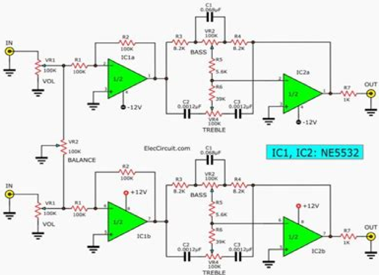
High Gain Stereo Preamplifier with Tone control
