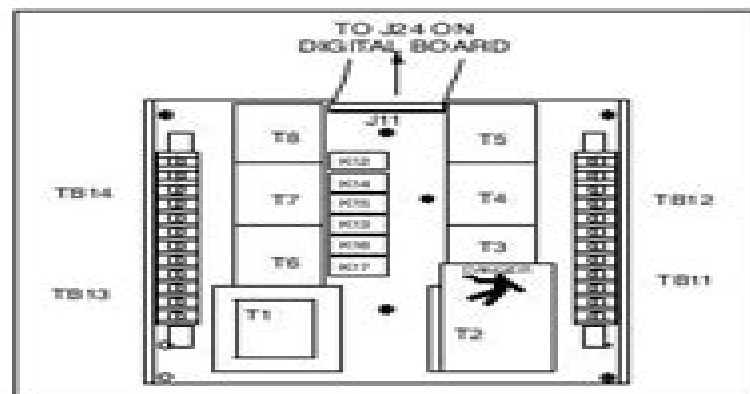
FIGURE 2-12. POWER MODULE
