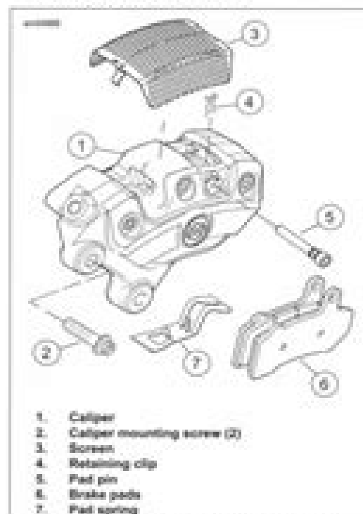
Figure 3-47. Front Brake Caliper Assembly
