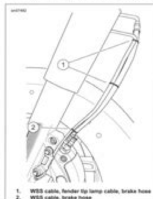
Figure 3-48. Secure Cables and Brake Hose
