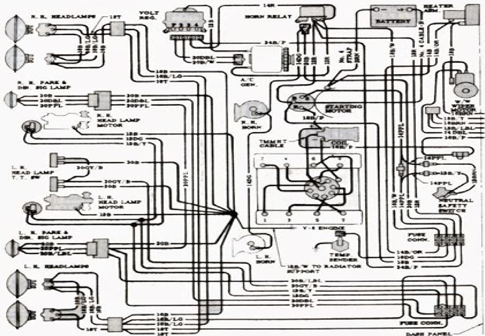
Engine compartment wiring, Corvette, 1965.
