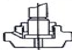
PRESSURE RELIEF PLUG (DN125 & ABOVE)
