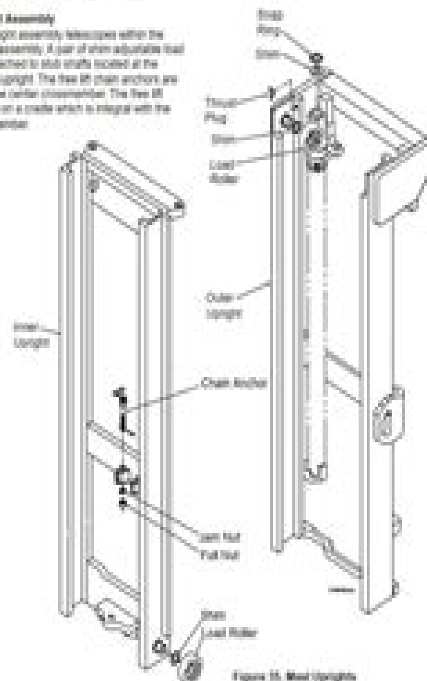
Figure 15. Mast Uprights
