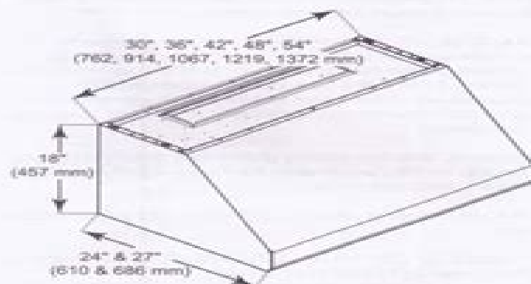
Figure 1: 24" & 27" Wall Hood Overall Dimensions
