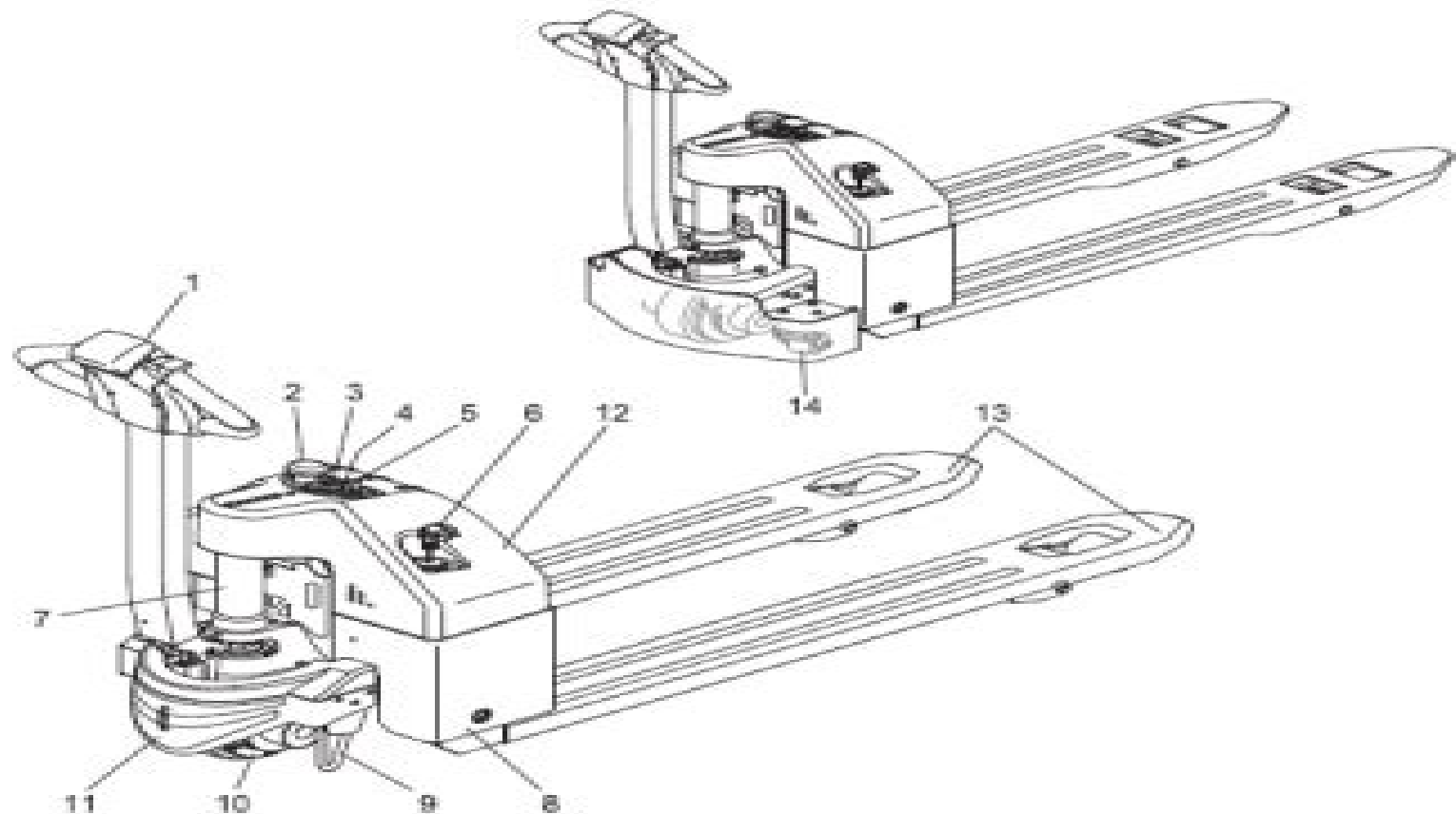
Figure 1-2 Lift Truck
