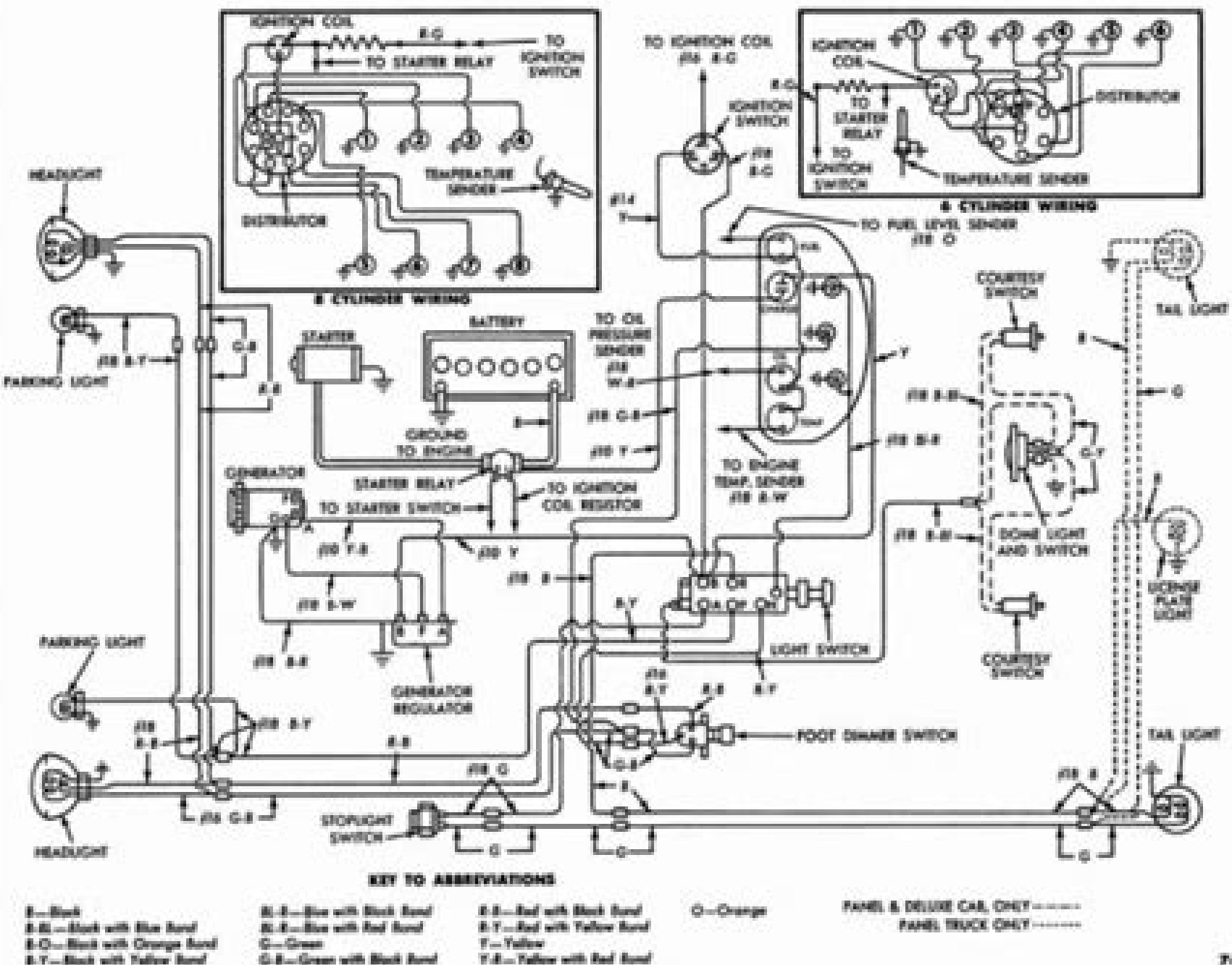
Fig. 1—Truck Wiring Diagram
