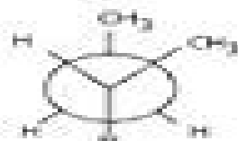
n-Butane
