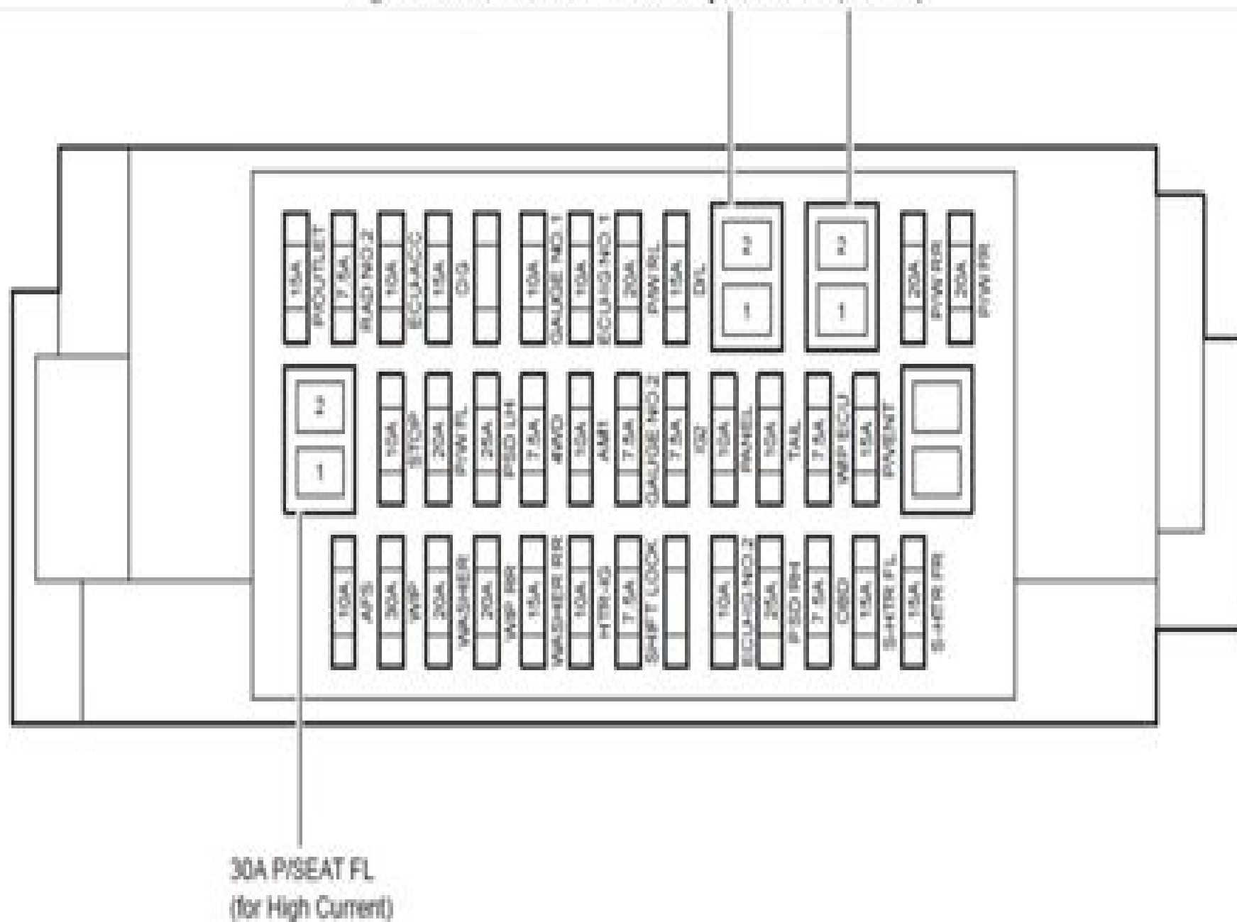
Fig. 17: Instrument Panel J/B Relay Locations (View C)
