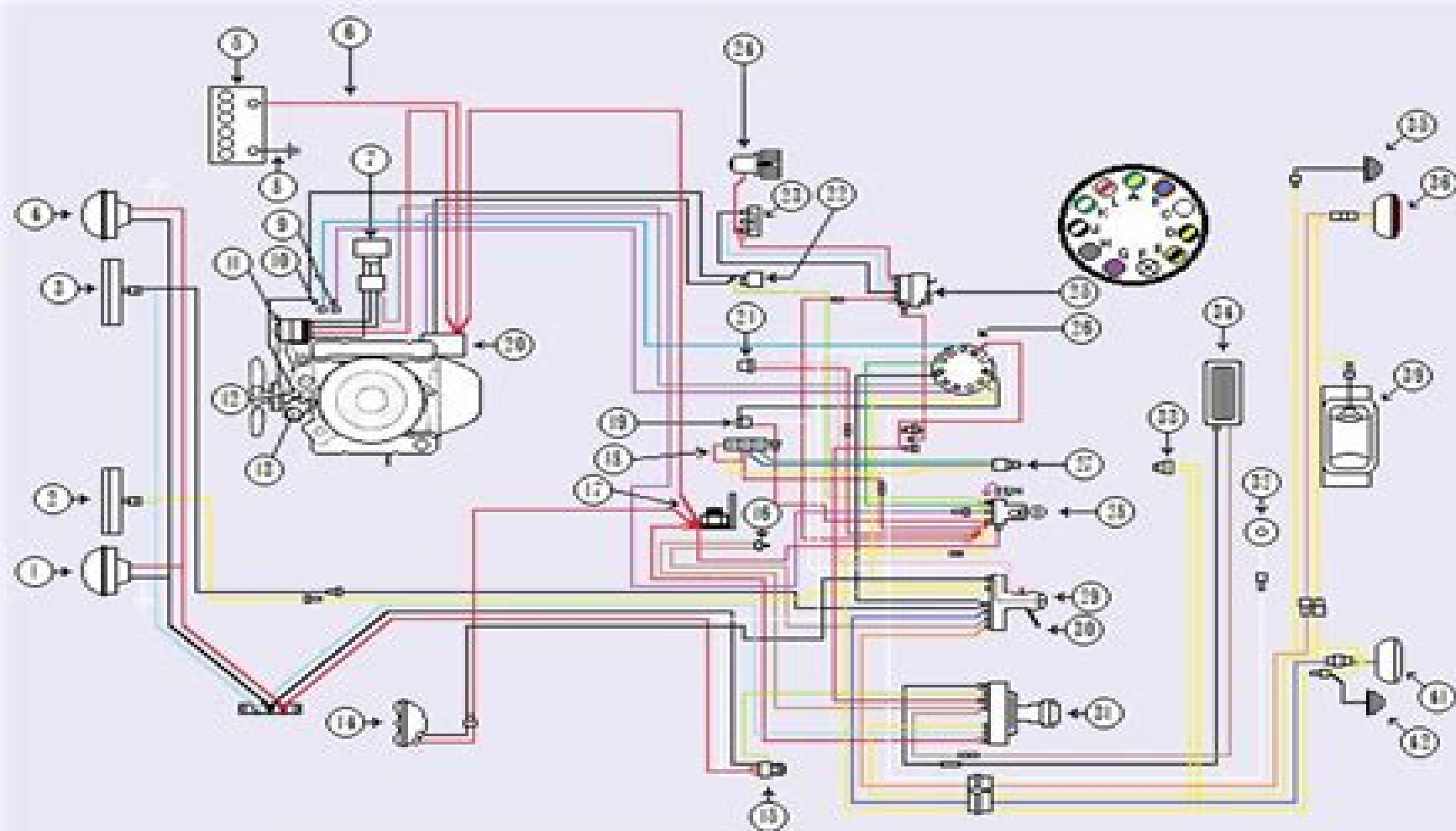
FIG. H-71—WIRING DIAGRAM, GLADIATOR TRUCK WITH V8-350 ENGINE
