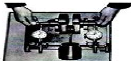
Fig. 6-2-11 Inspection crankshaft deflection
