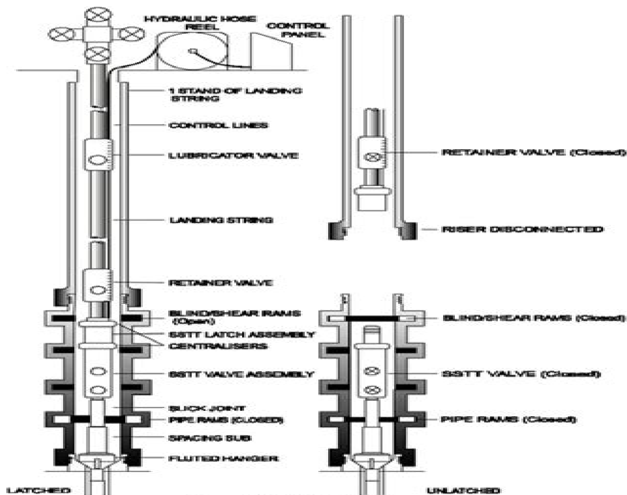
Figure 5.A - SSTT Arrangement
