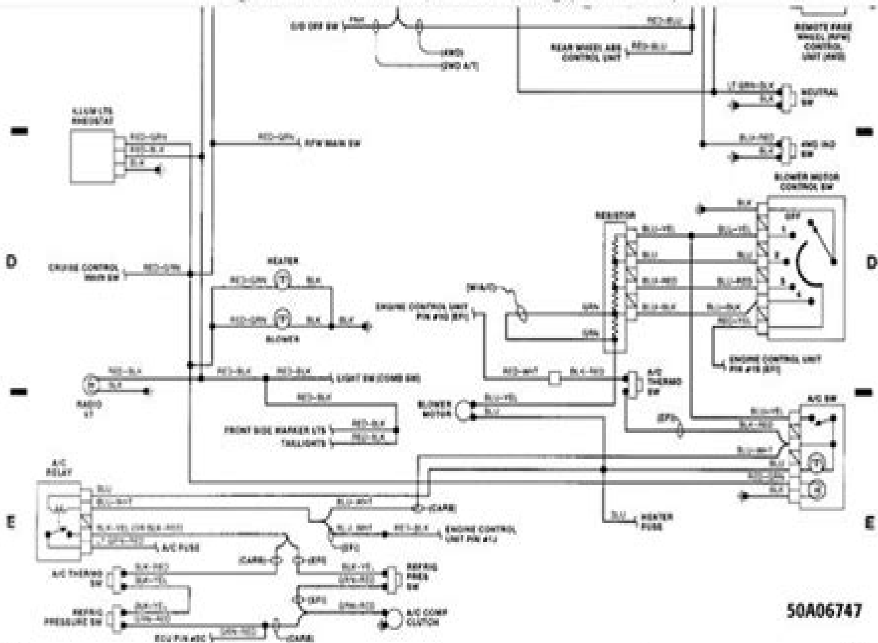
Fig. 5: Instrument Panel, A/C &amp; Heating (Grids 16-19)
