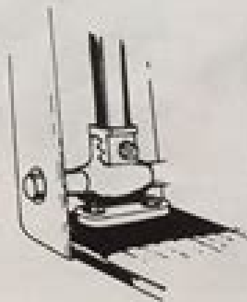
FIG. 15. BOTTOM END OF TUBULAR FRAME ASSEMBLY
