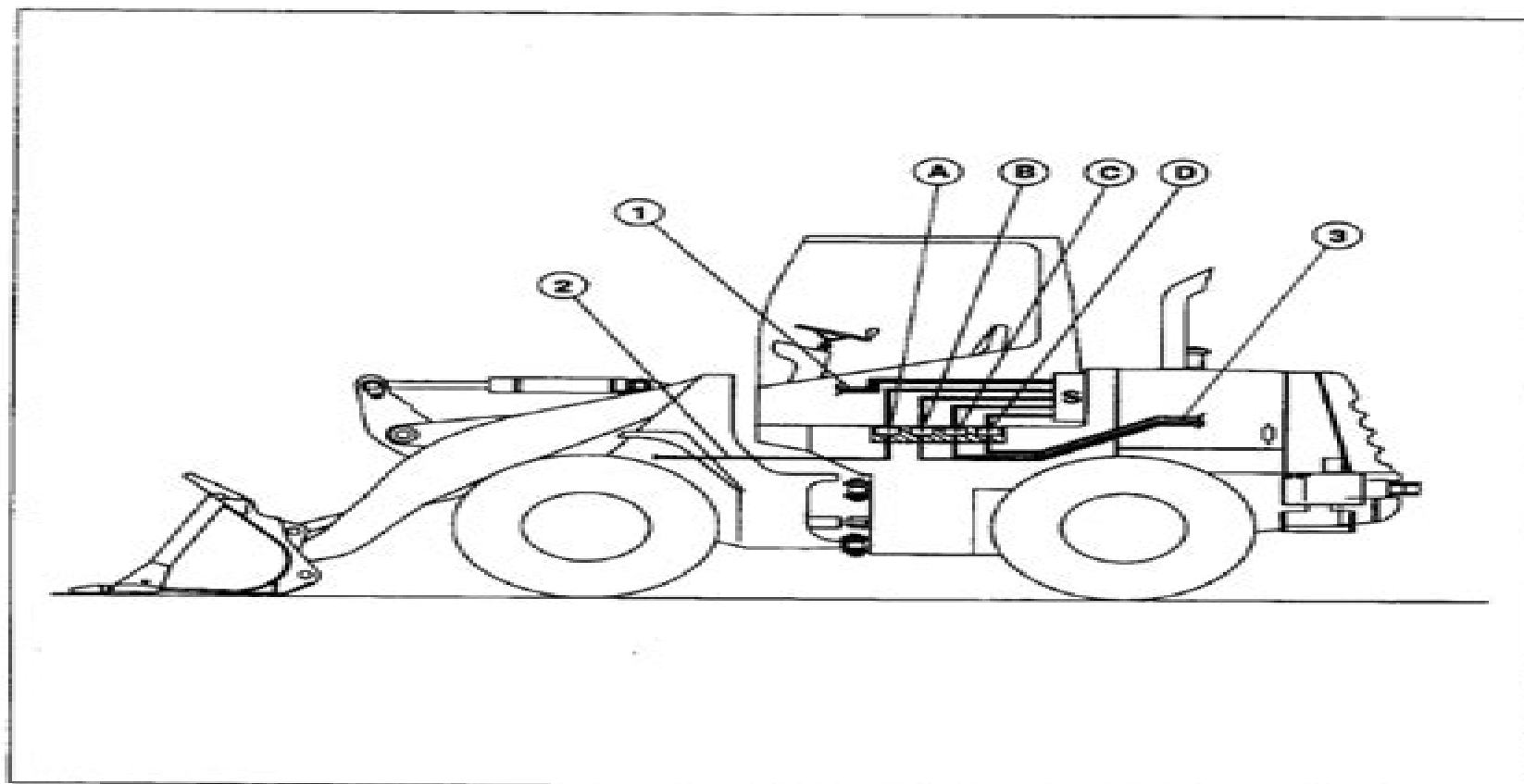
A-B-C-D. Connectors - S. Logic board - 1. Cab wiring - 2. Front frame wiring - 3. Rear frame wiring.
