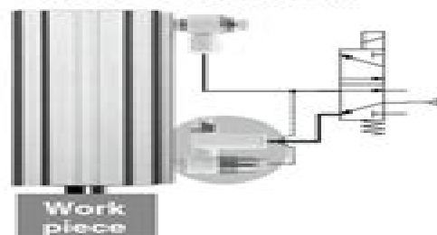
Example of drop prevention circuit
