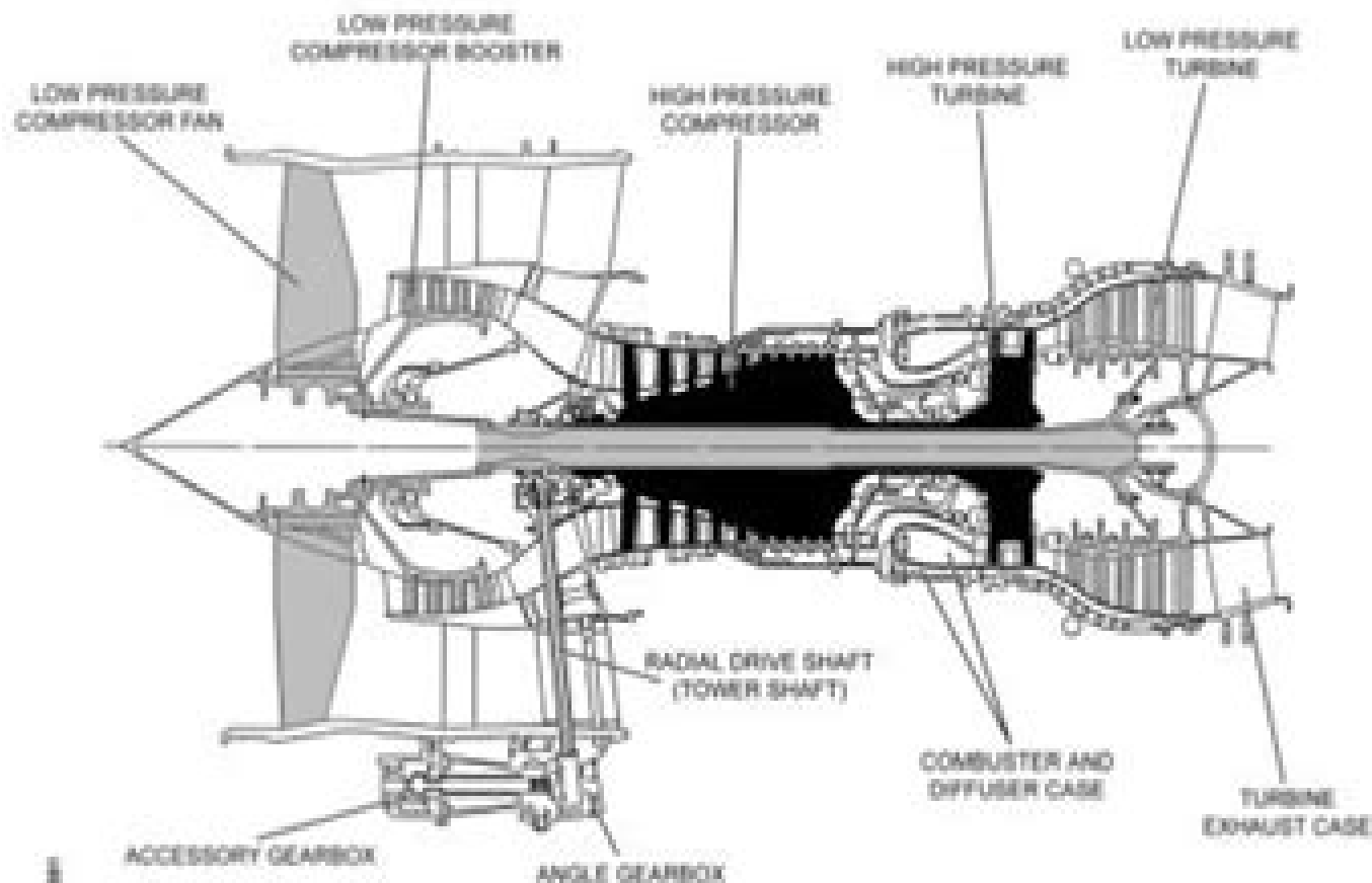
ENGINE GENERAL ARRANGEMENT
