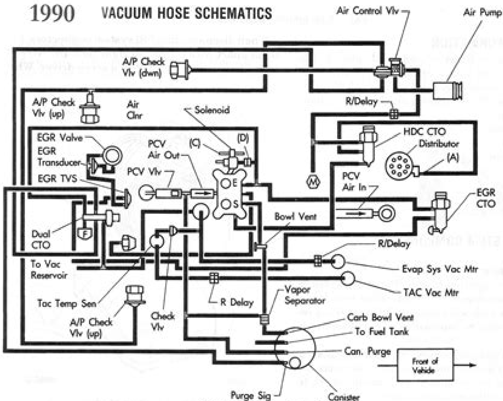
SJ Vacuum Routing Schematic
