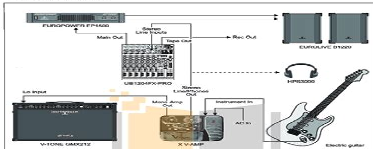
Fig. 3.1: Standard application (example)
