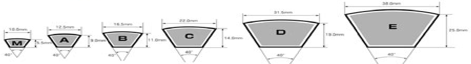
Belt Cross-Section Dimensions:
