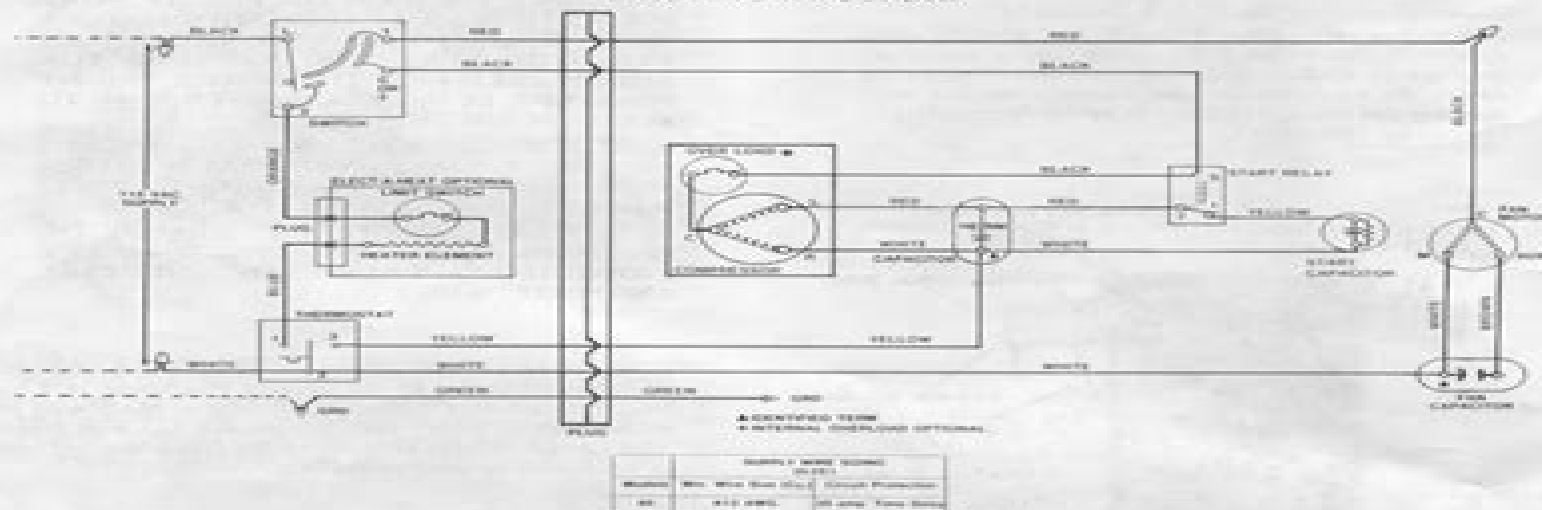
LADDER TYPE WIRING DIAGRAM
