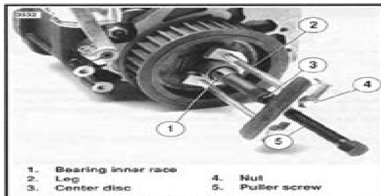
Figure 7-15. Pull Mainshaft Inner Bearing Race
