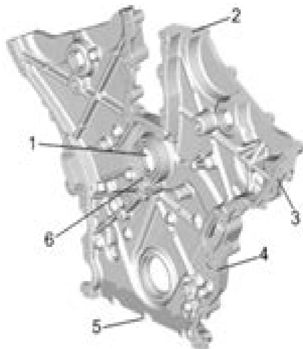
Fig. 41: Identifying Interior Of Engine Front Cover Inspection Locations Courtesy of GENERAL MOTORS COMPANY
