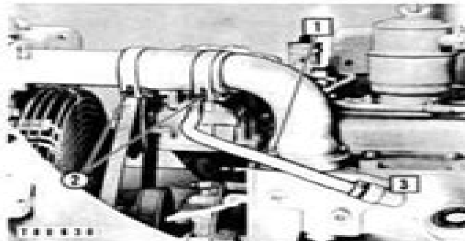
PREPARING TO REMOVE TEMPERATURE REGULATOR 1-Valve (two), 2-Hose clamps, 3-Elbow.
