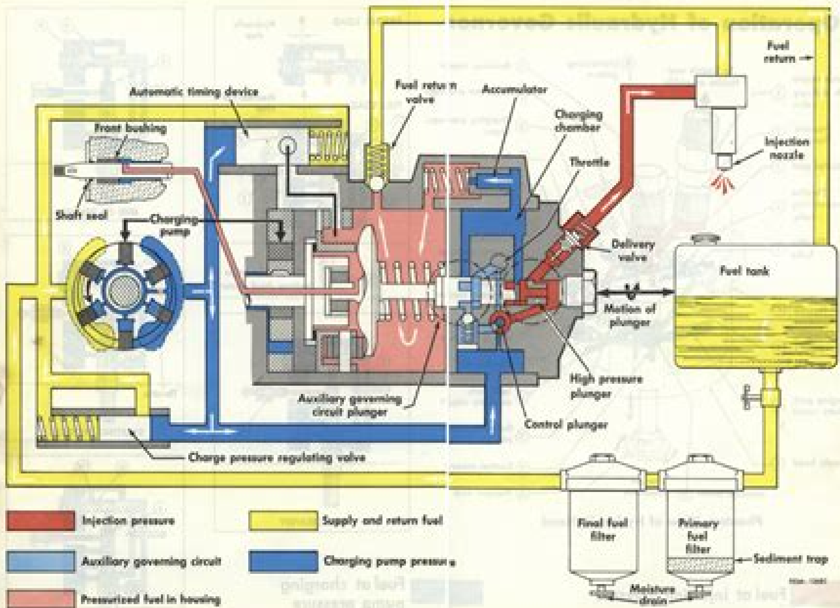
Illustr. 2-7. Fuel flow diagram.
