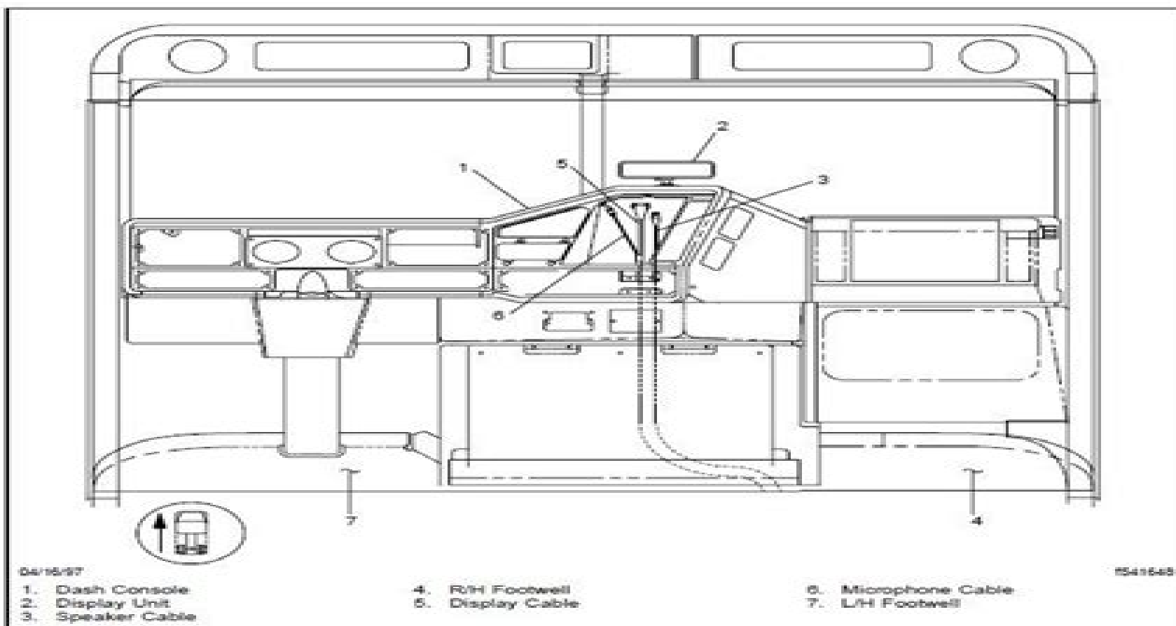
Fig. 3, Display and Microphone Cable Routing (dash)
