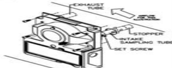
FIGURE 2. FCD-350 MOUNTING
