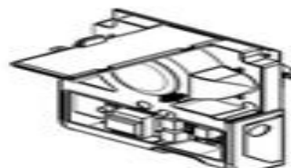
FIGURE 7. FCD-350 ACCESS HATCH COVER TEMPORARY STORAGE
