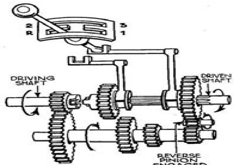
The separate reverse train of gears
