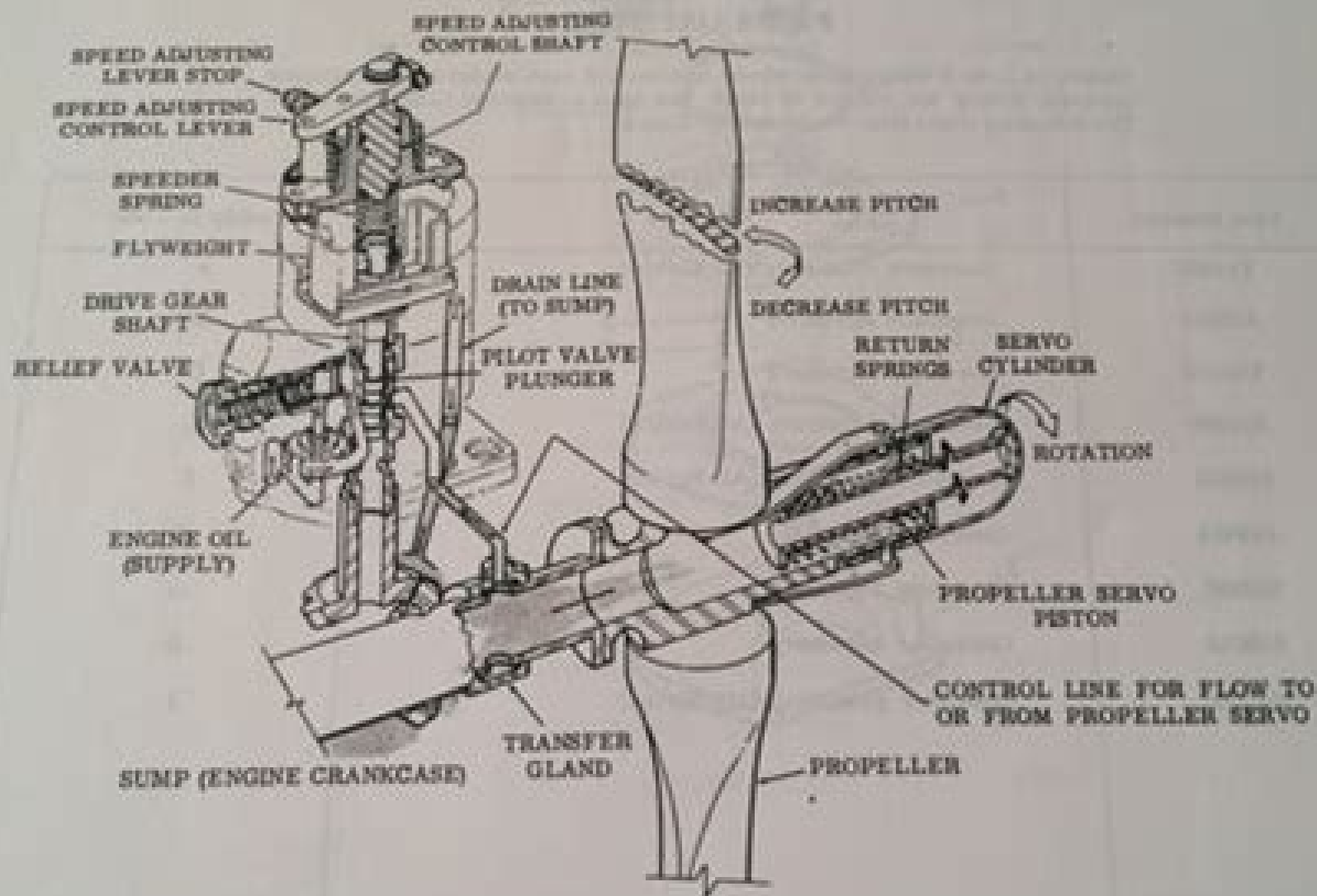
Figure 3. Schematic Diagram of Operation (Pressure to Increase Pitch Only)
