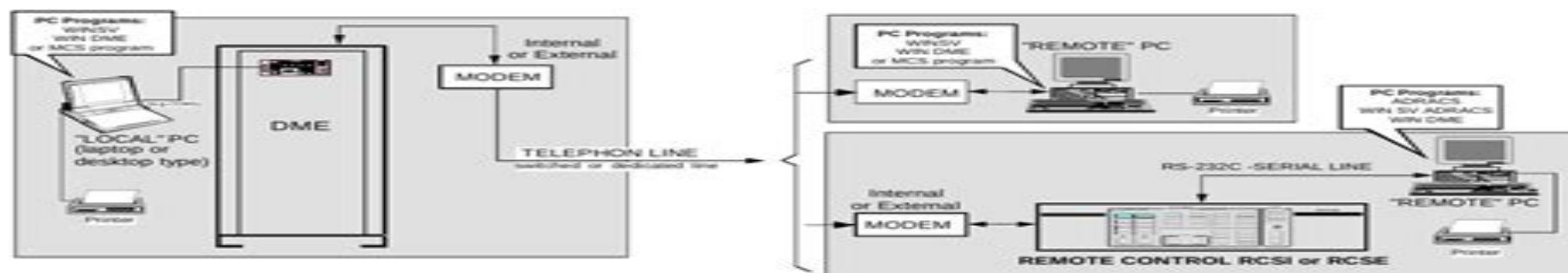
Figure 3.40. Examples of PC user programs with DME stand alone
