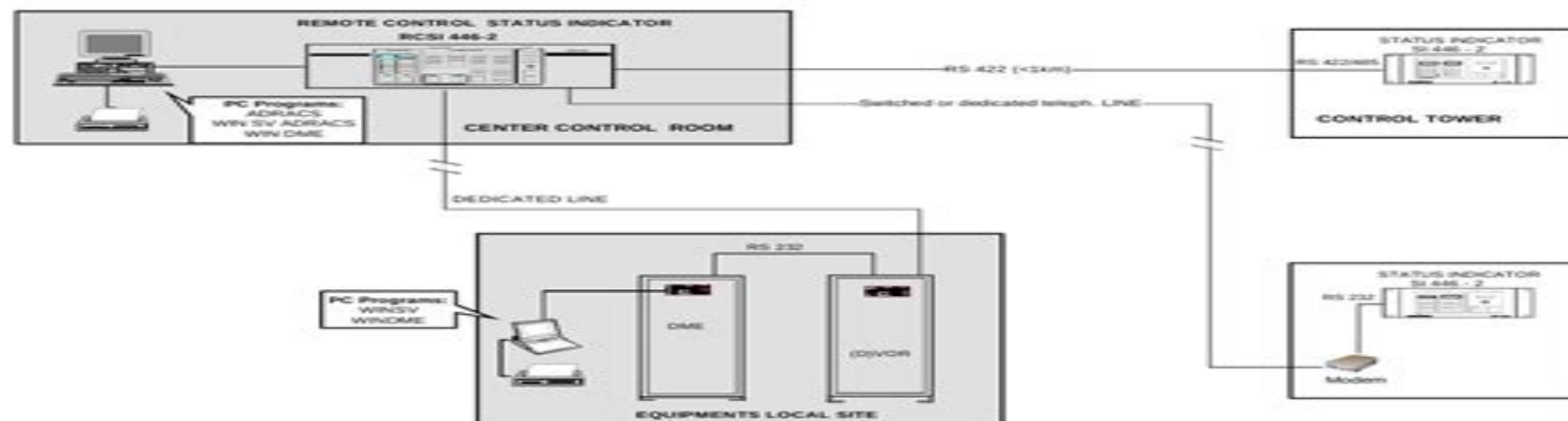
Figure 3.41. Examples of PC user programs in VOR-DME system
