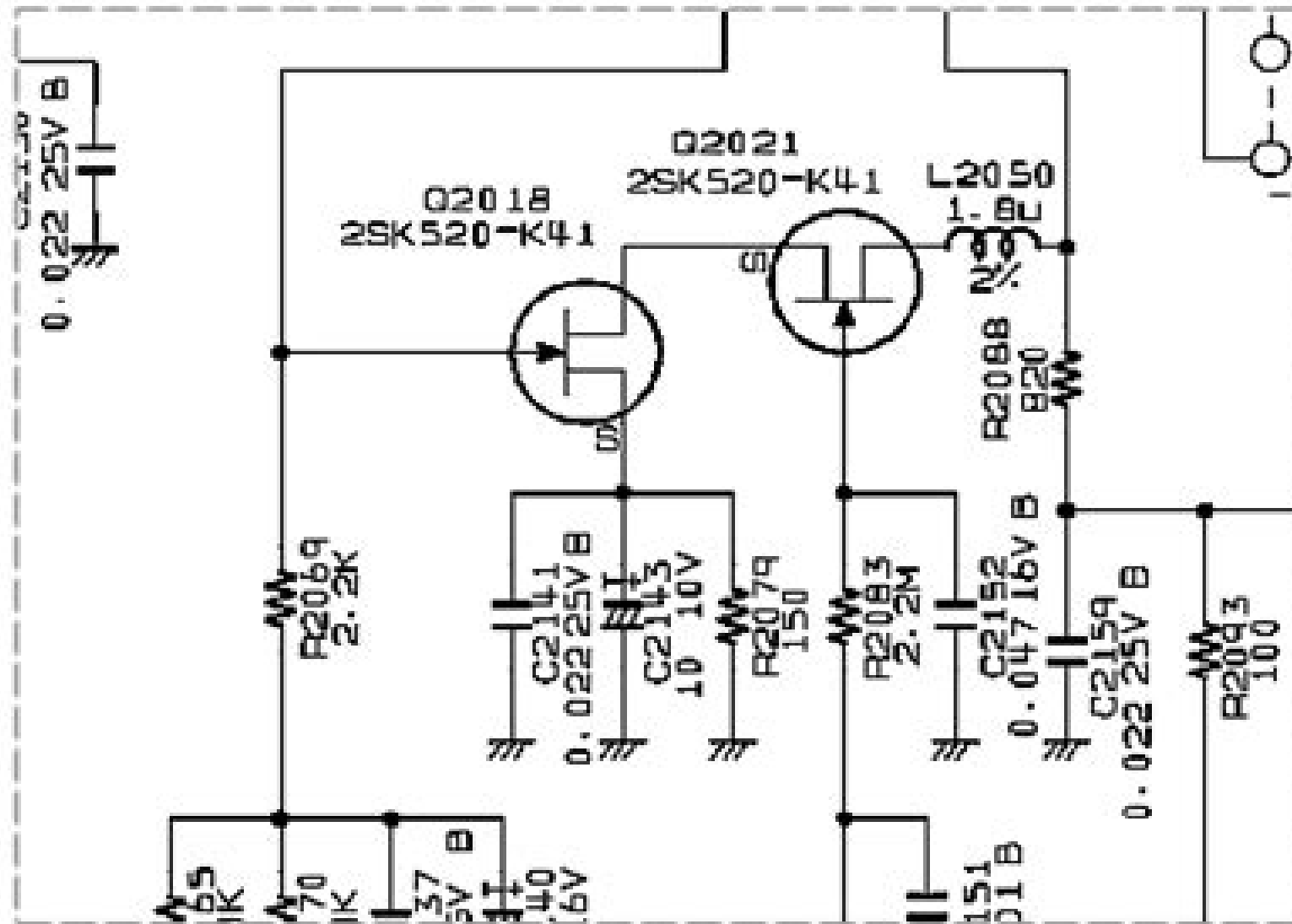
Preview: YAESU FT-450 schematic diagram
