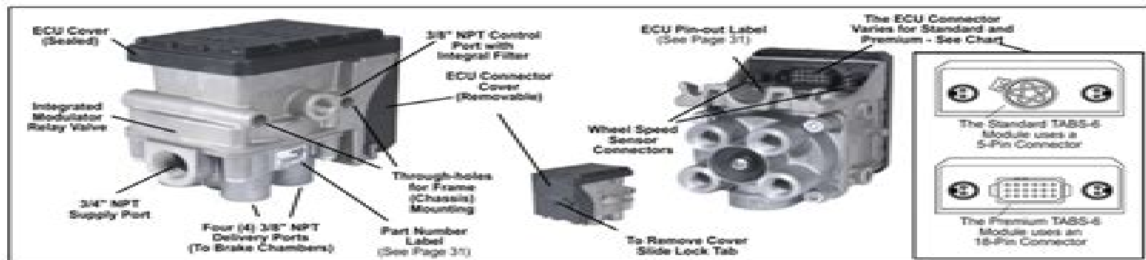
FIGURE 1 - TABS-6 STANDARD AND PREMIUM MODULES
