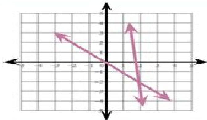
Independent System
