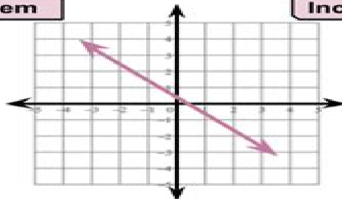
Dependent System
