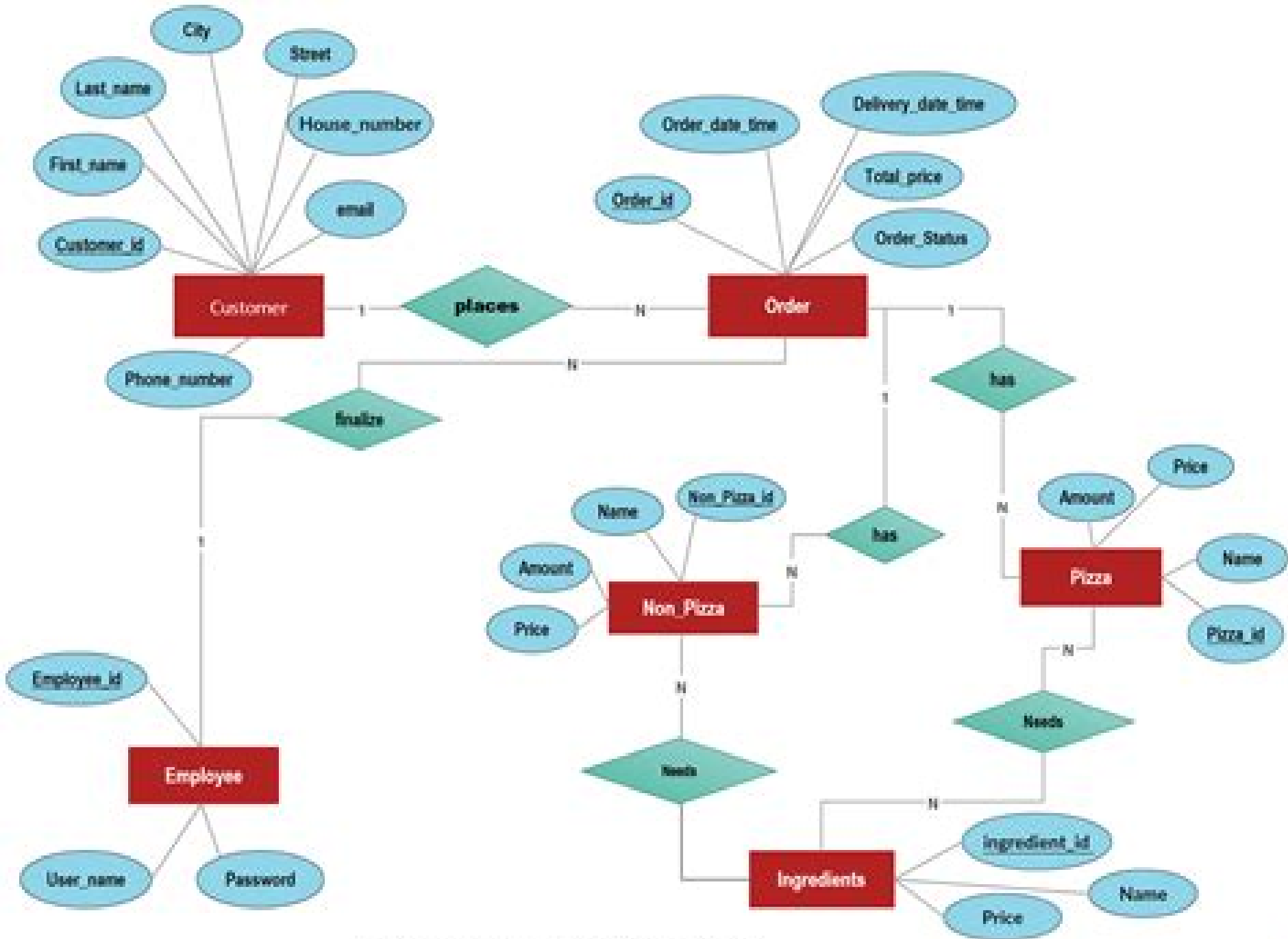
ER Diagram: Online Pizza Ordering System
