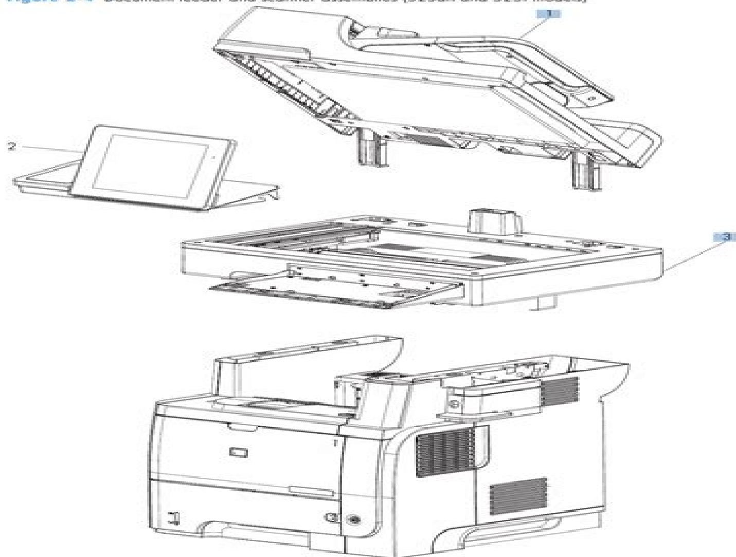
Figure 2-4 Document feeder and scanner assemblies (525dn and 525f models)
