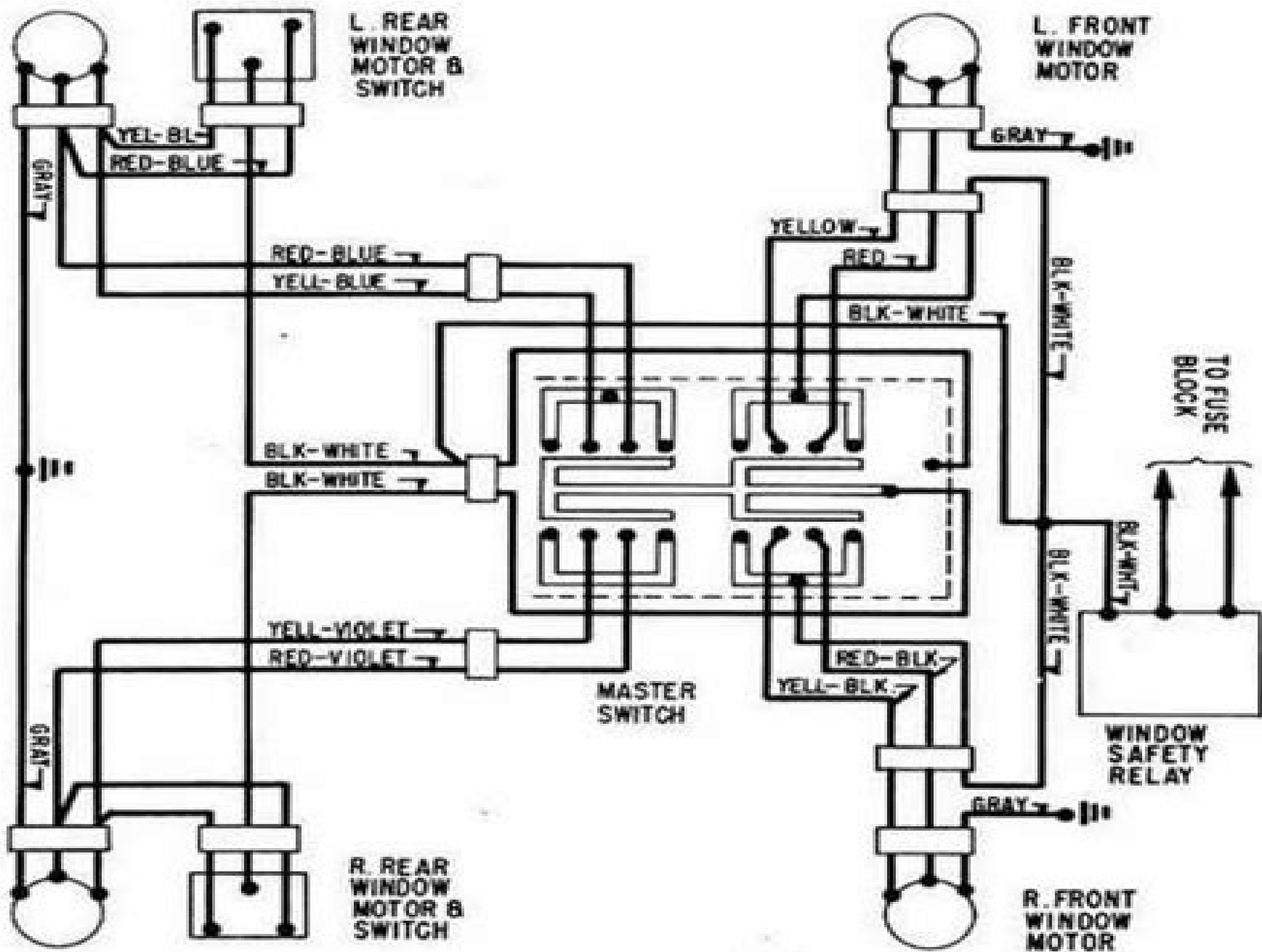
1965 THUNDERBIRD
