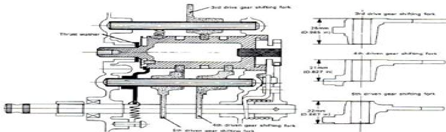
Fig. 6-2-31 Gear shifting forks
