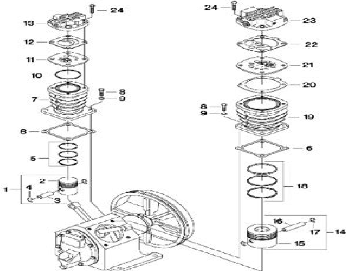
FIGURE 4. MODEL 347 1/2 INCH COMPRESSOR PUMP.
