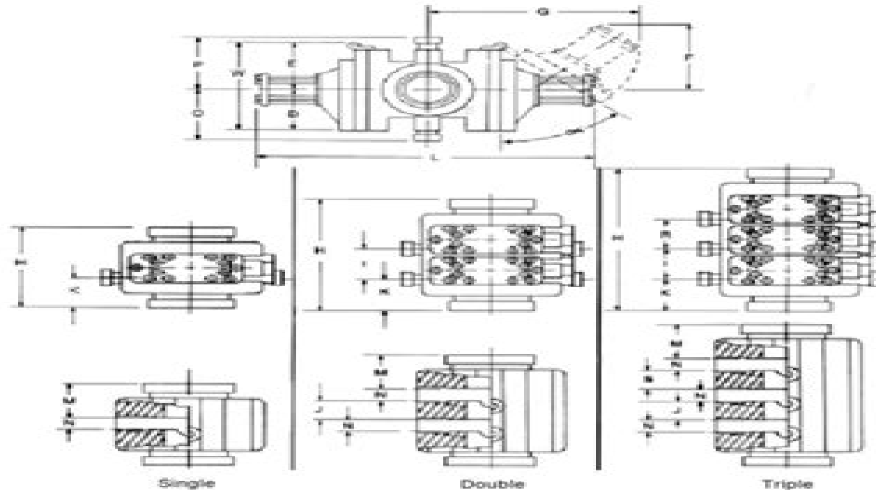
Figure 4-1 Model SL BOPs—Dimensions and Specifications
