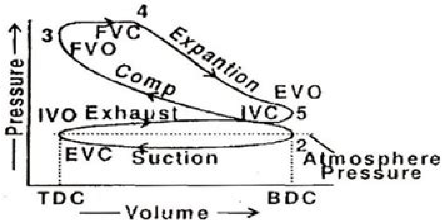
Indicator diagram for a Four Stroke Cycle Diesel Engines.
